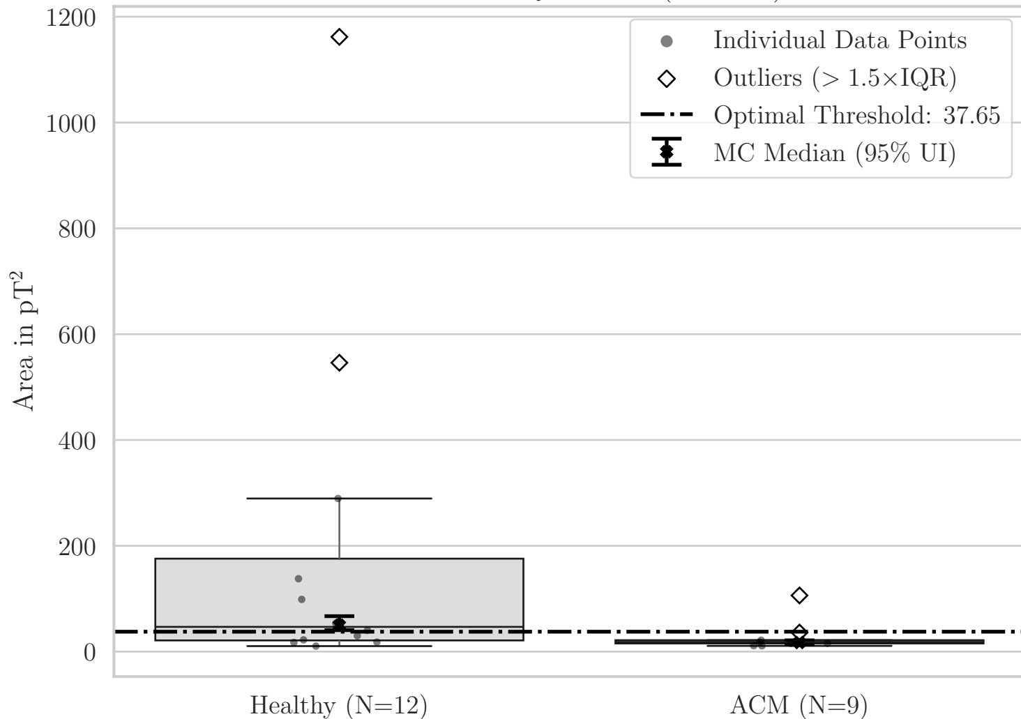
Box Plot for QRS Area (OW YZ)
