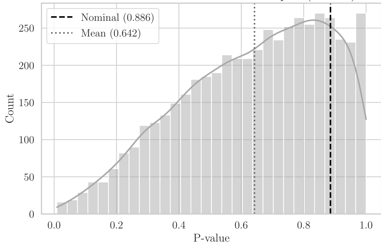
MC Distribution of P-values for ST Compact (OX XY)
