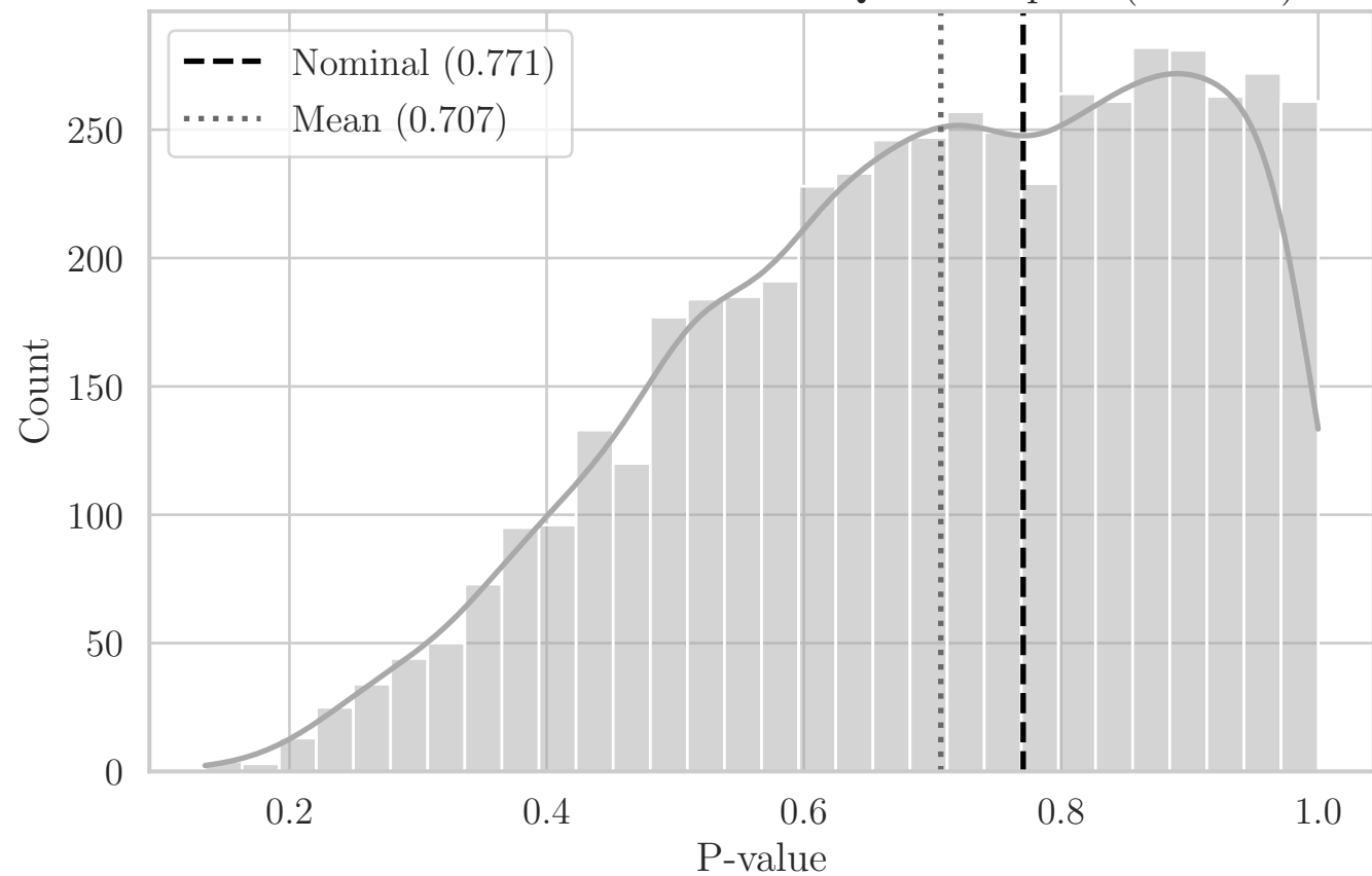
MC Distribution of P-values for QRS Compact (OY XY)
