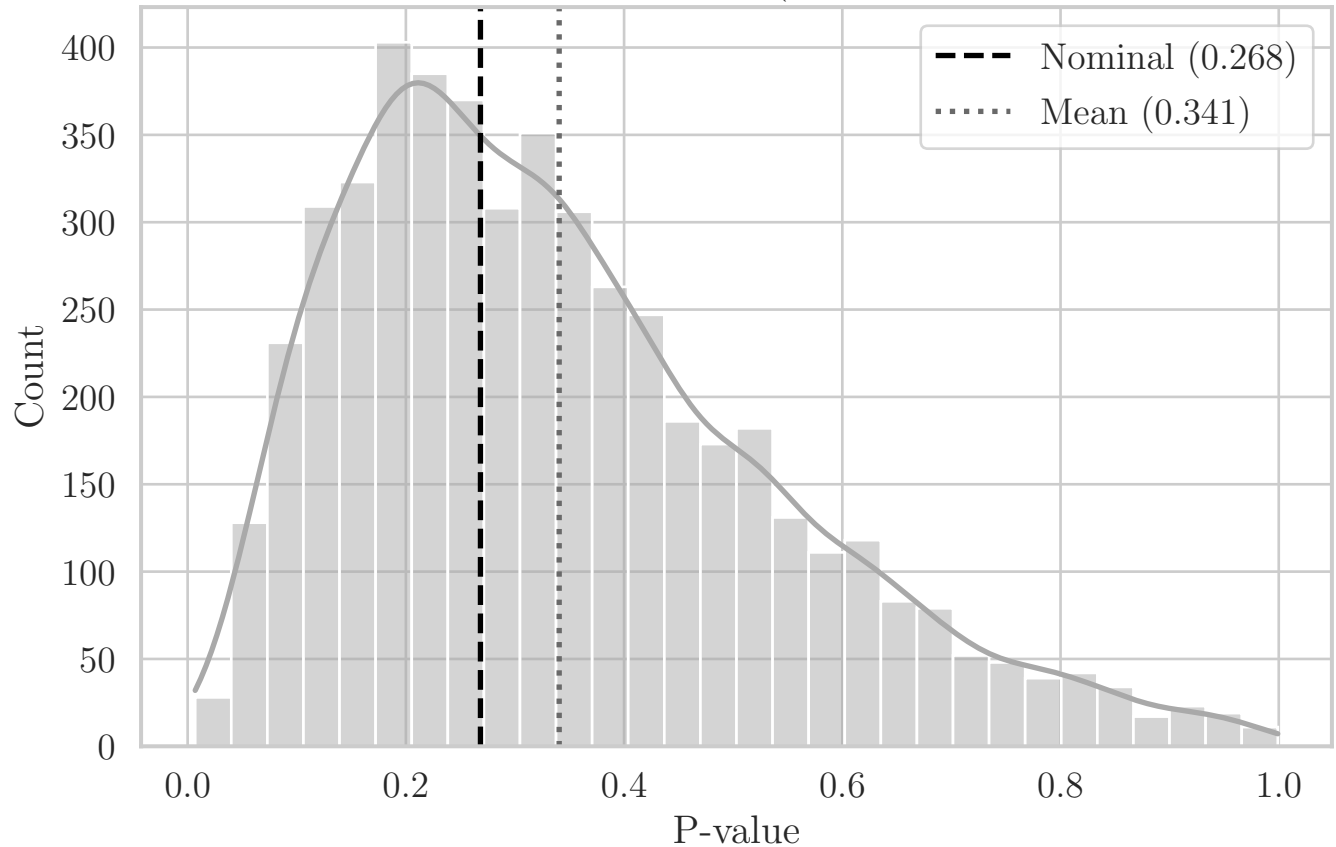
MC Distribution of P-values for T Compact (Aggregated Bottom-Left Quadrant XY)
