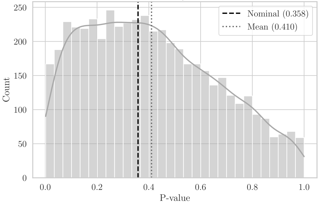
MC Distribution of P-values for ST Angle (Aggregated Bottom-Left Quadrant YZ)
