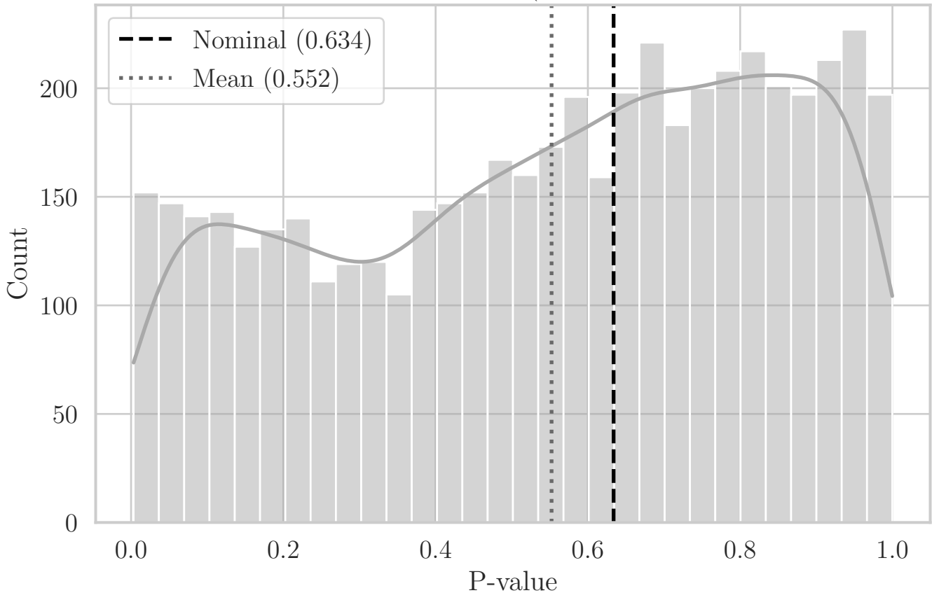
MC Distribution of P-values for QRS Angle (Aggregated Bottom-Right Quadrant XY)
