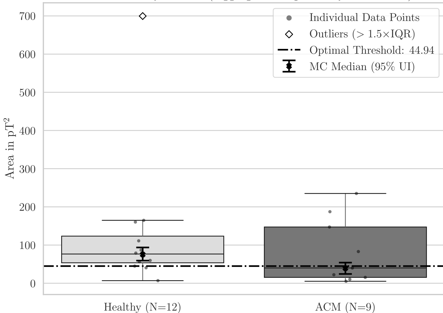
Box Plot for QRS Area (Aggregated Top-Left Quadrant XY)
