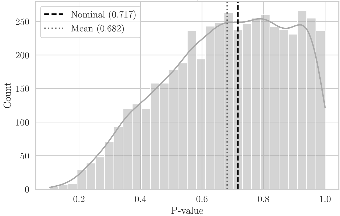
MC Distribution of P-values for T Angle (Aggregated Top-Right Quadrant XY)
