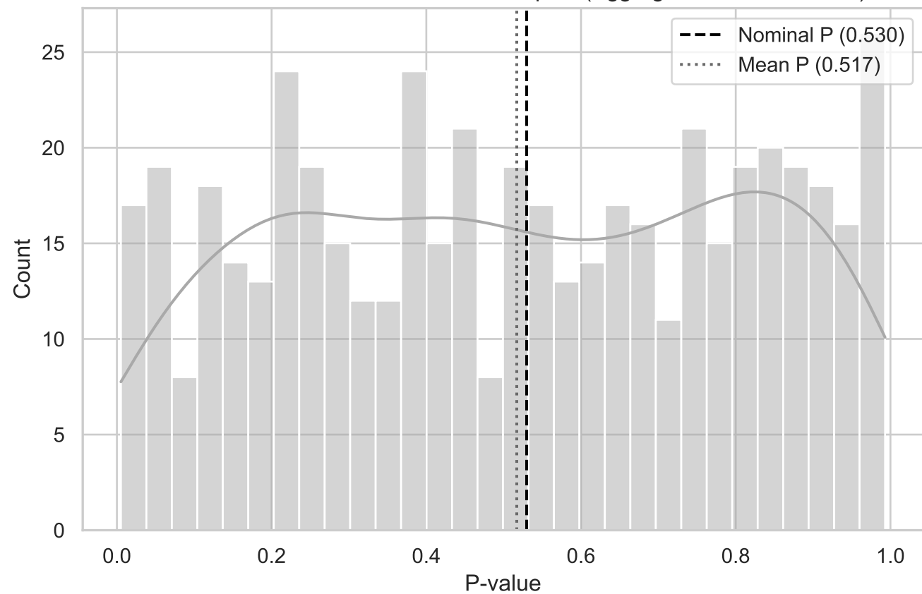
MC Distribution of P-values for ST Compact (Aggregated BottomLeft YZ)
