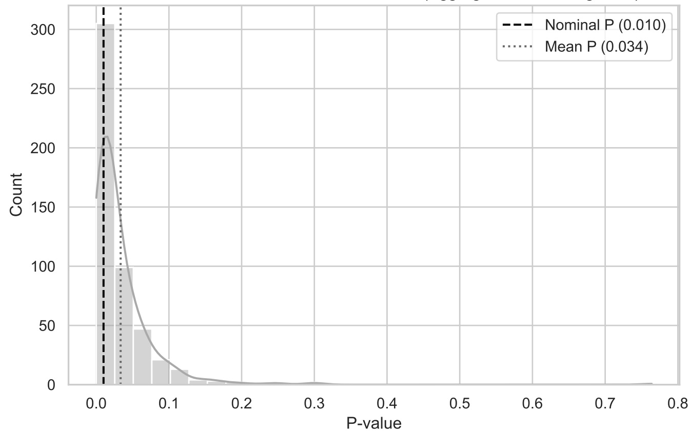
MC Distribution of P-values for QRS T-Dist (Aggregated BottomRight XY)
