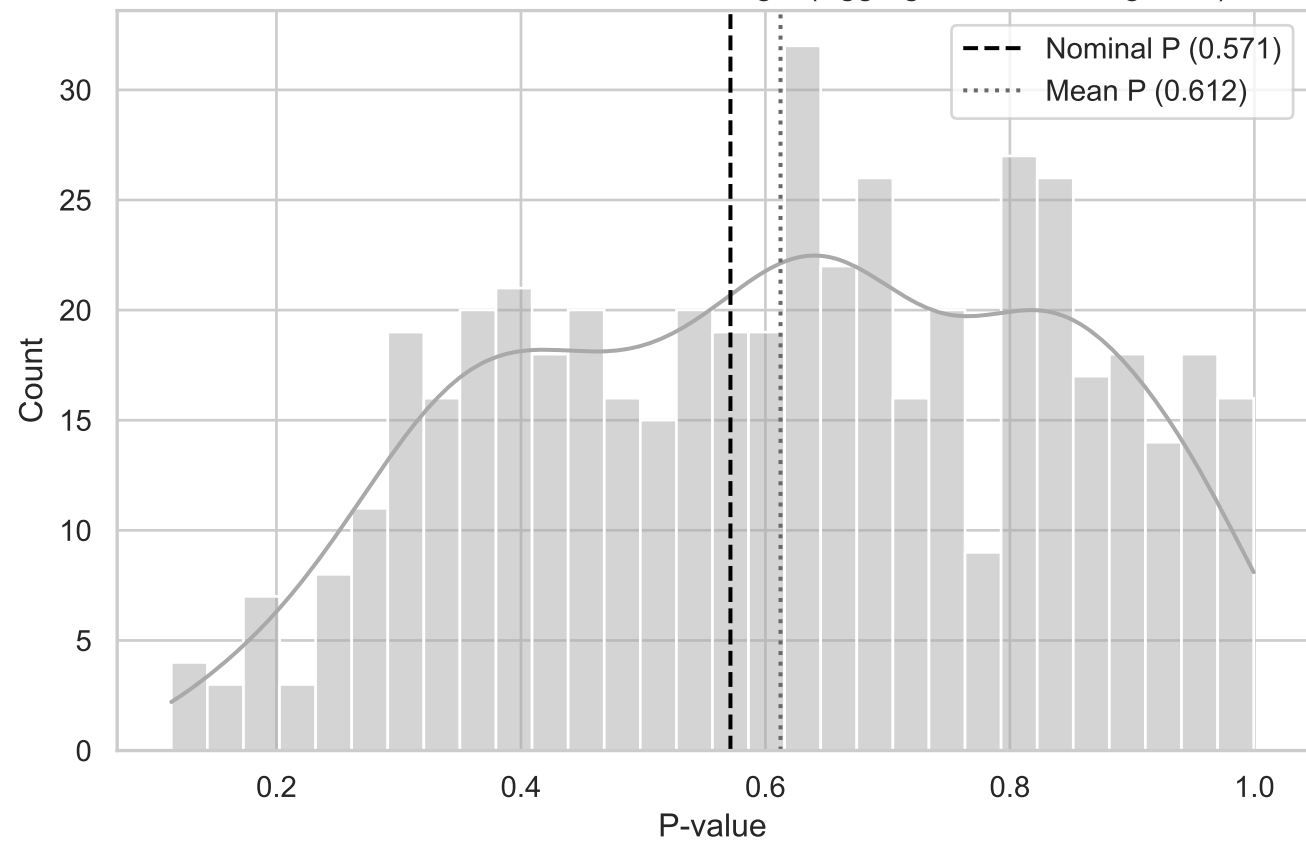
MC Distribution of P-values for QRS Angle (Aggregated BottomRight YZ)
