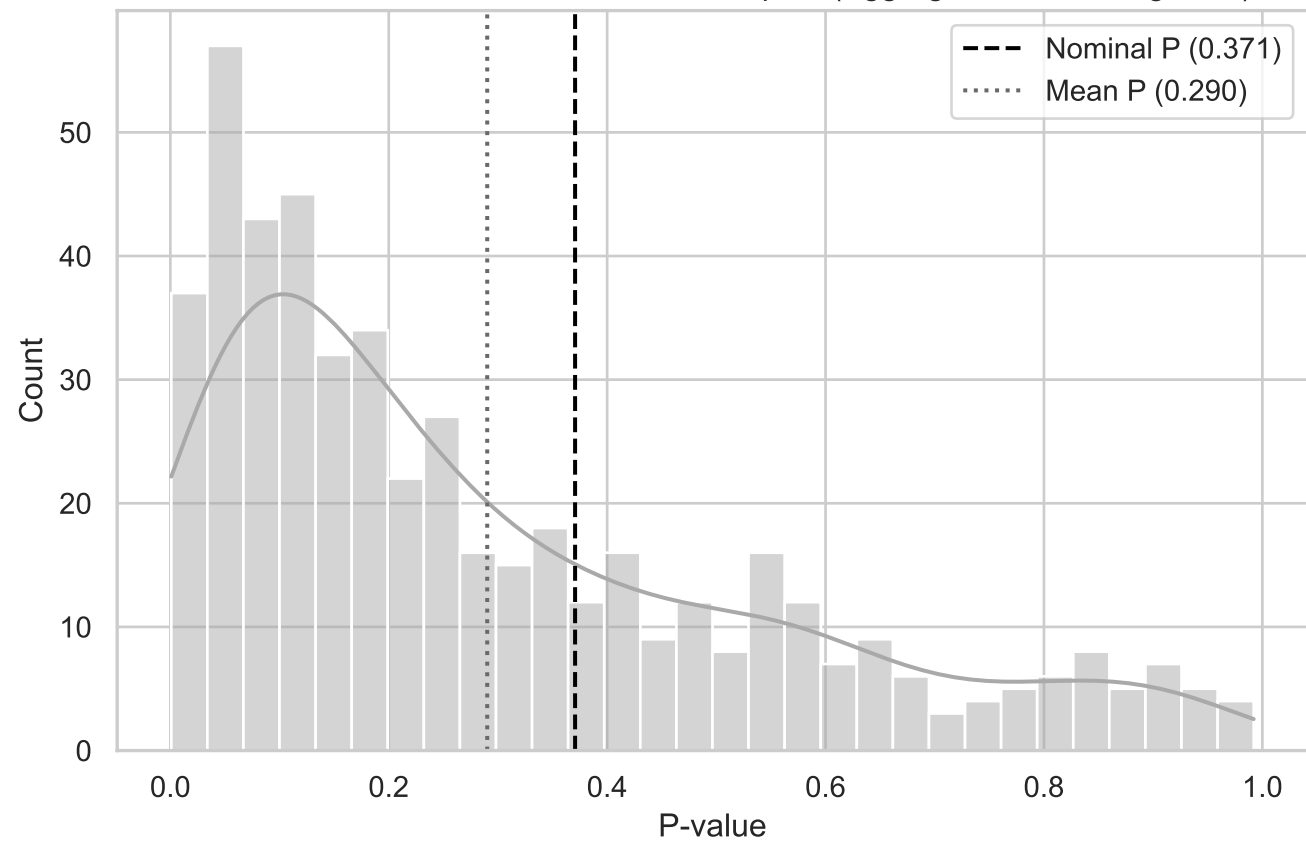
MC Distribution of P-values for QRS Compact (Aggregated BottomRight YZ)
