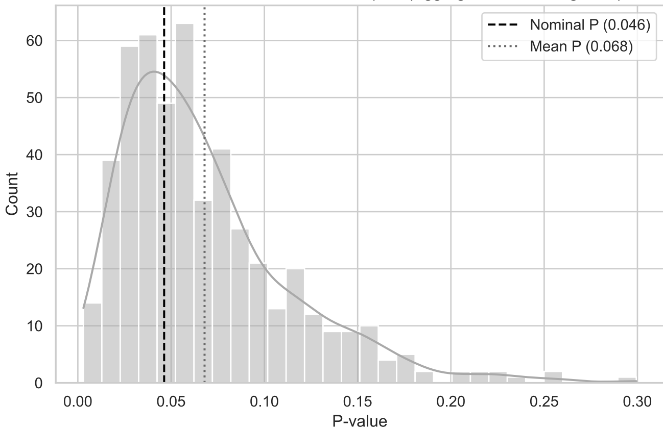
MC Distribution of P-values for T Compact (Aggregated BottomRight YZ)
