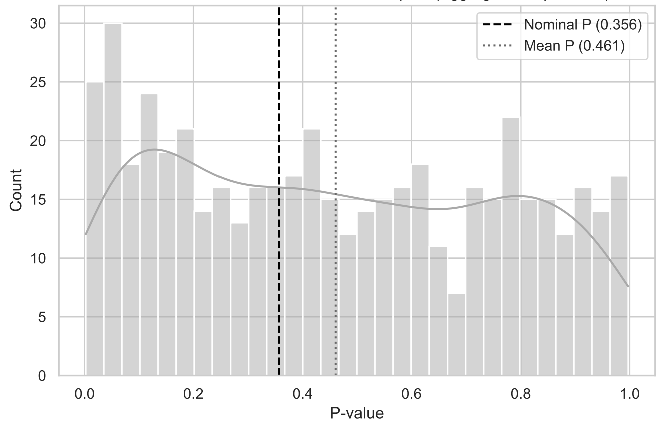
MC Distribution of P-values for QRS Compact (Aggregated TopLeft XY)
