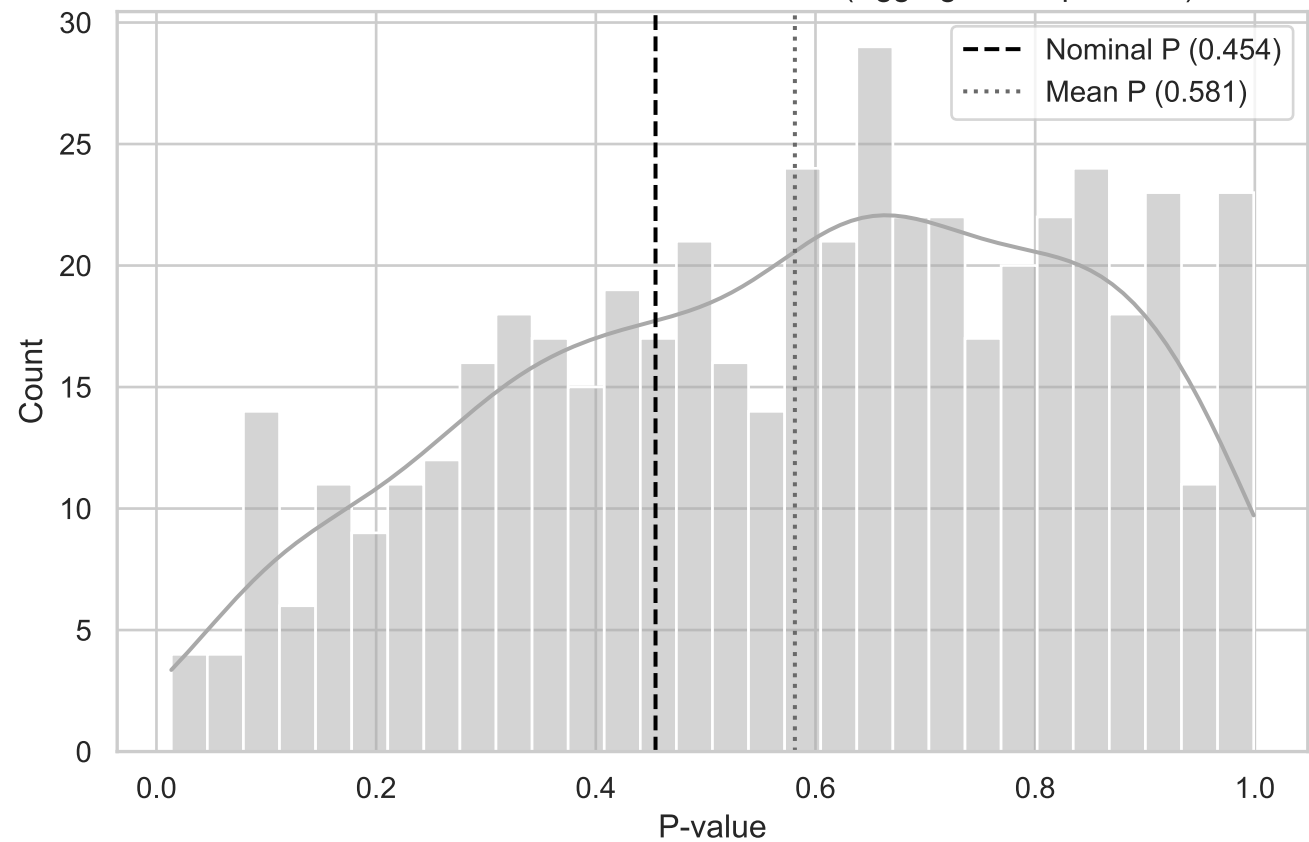
MC Distribution of P-values for QRS T-Dist (Aggregated TopLeft XY)
