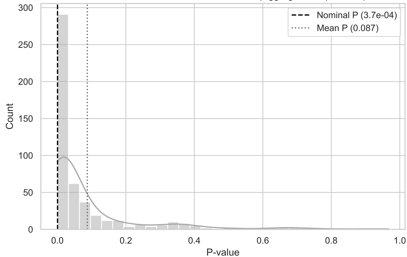
MC Distribution of P-values for ST T-Dist (Aggregated TopLeft XY)
