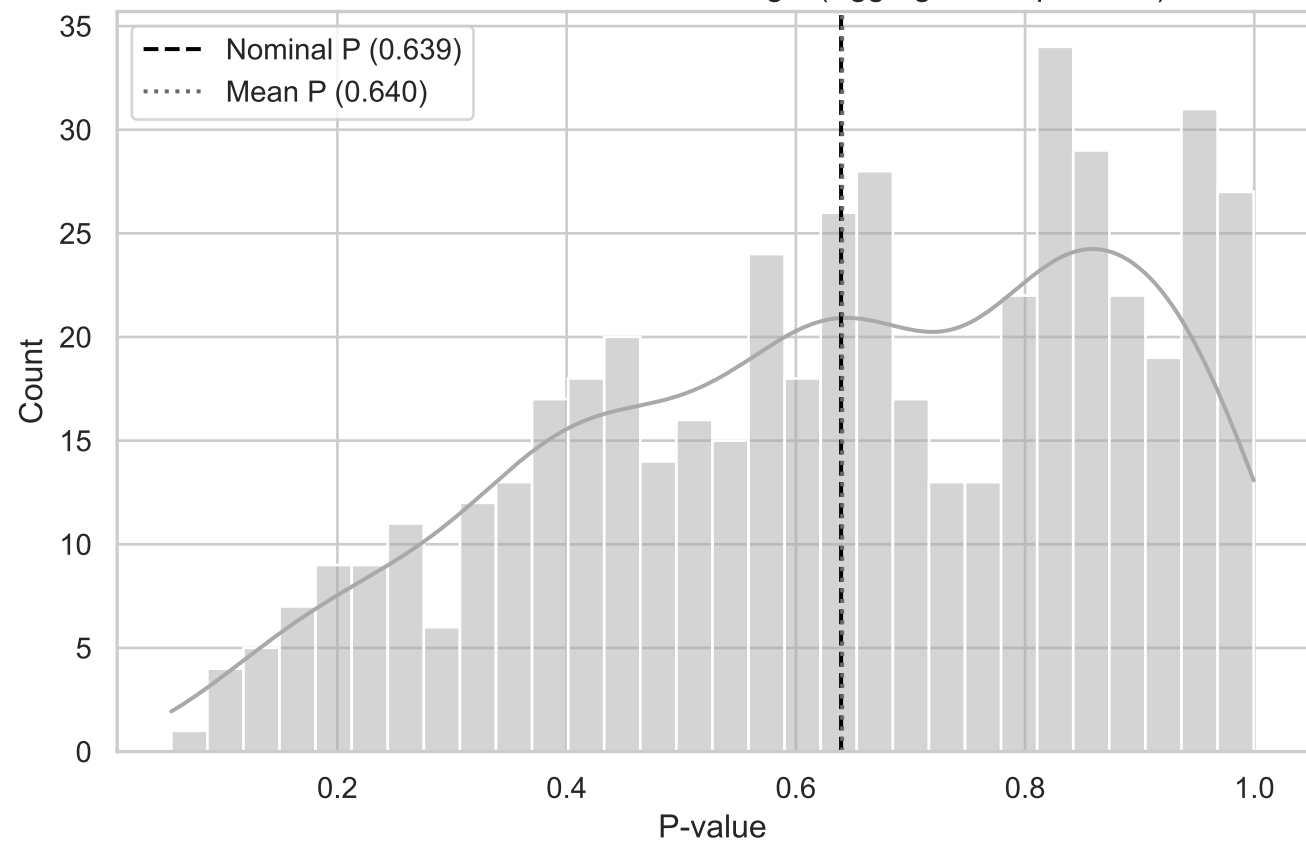
MC Distribution of P-values for T Angle (Aggregated TopLeft YZ)
