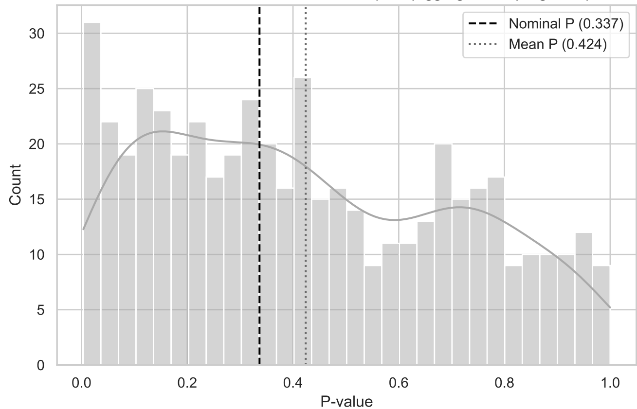
MC Distribution of P-values for ST Compact (Aggregated TopRight XY)
