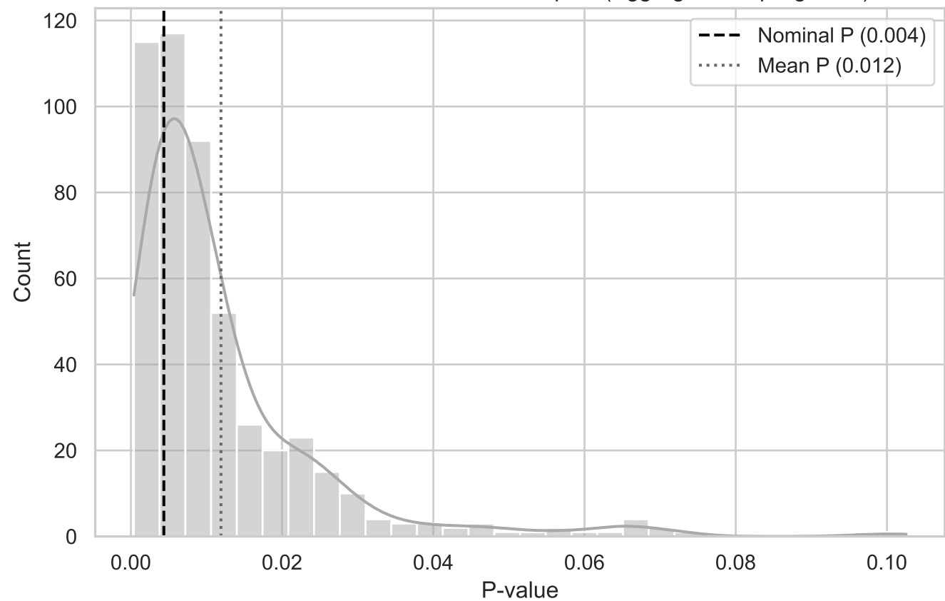
MC Distribution of P-values for T Compact (Aggregated TopRight XY)
