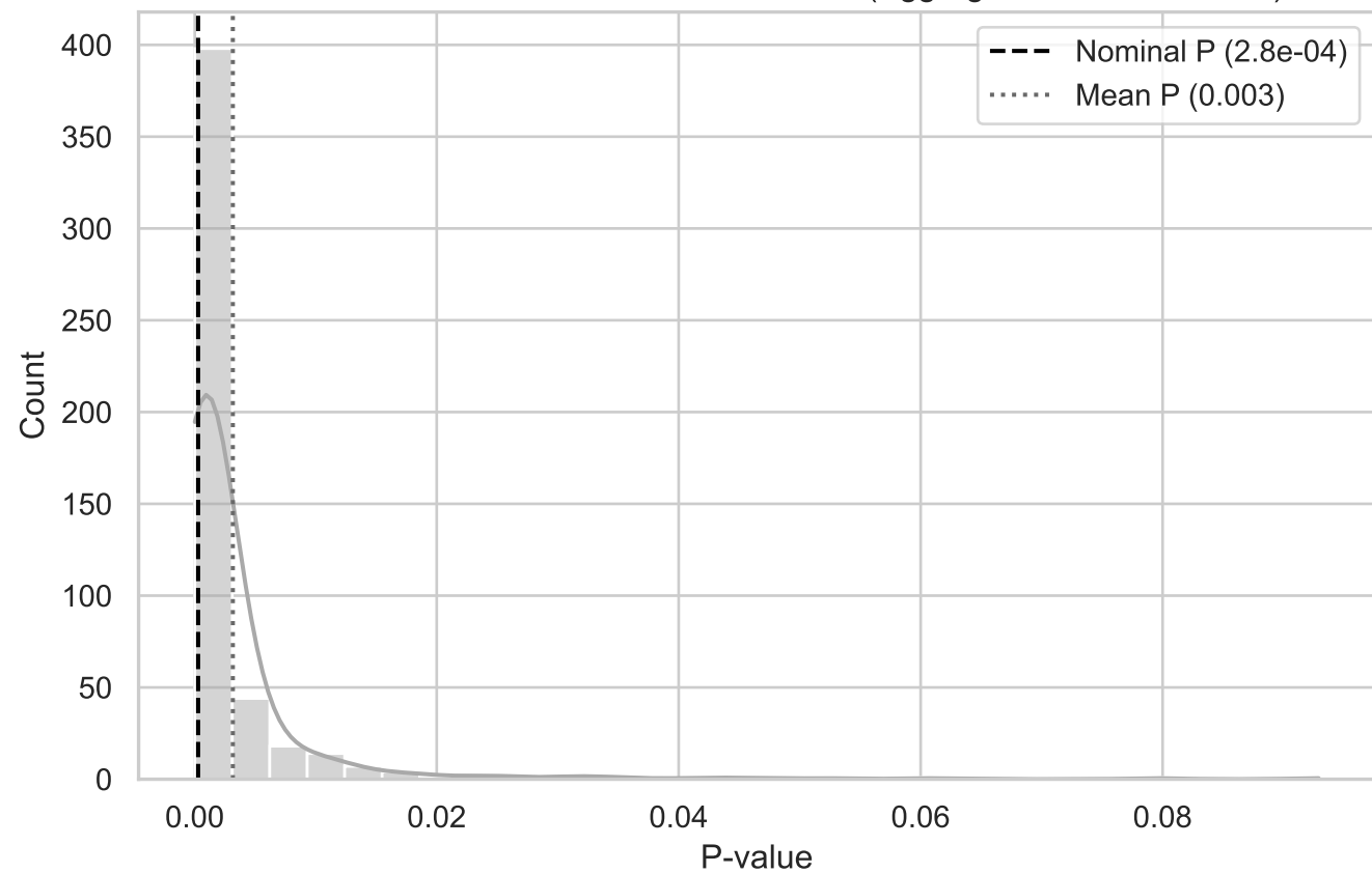
MC Distribution of P-values for QRS T-Dist (Aggregated BottomLeft XY)
