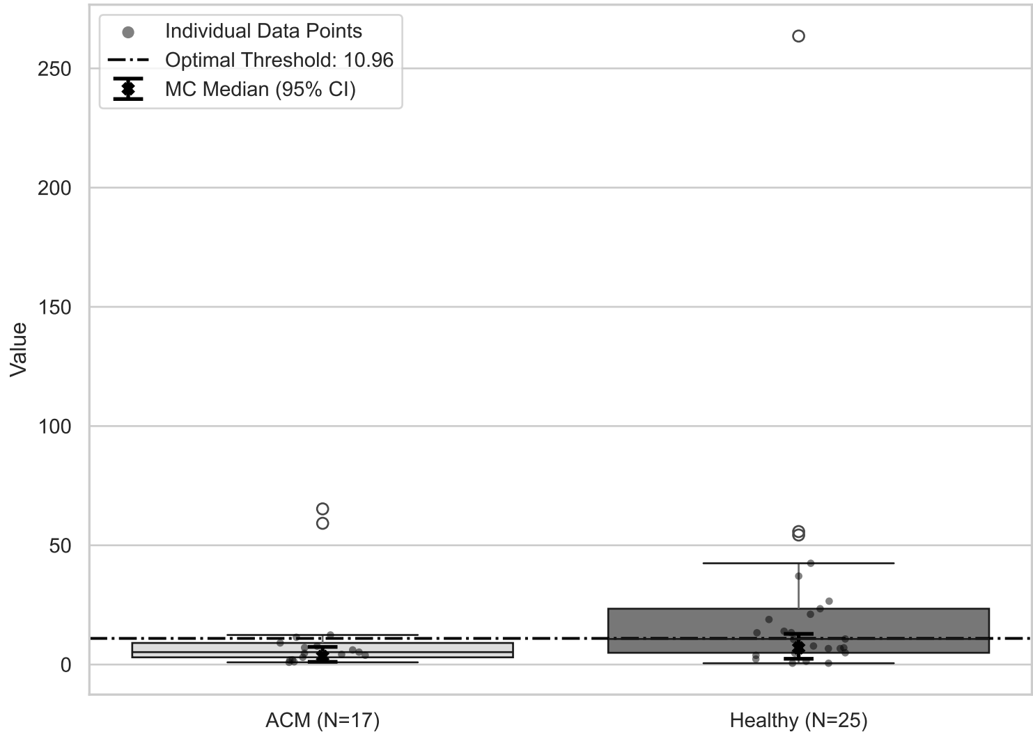
Box Plot of Nominal Data with MC Medians for ST Area (Aggregated BottomLeft YZ)
