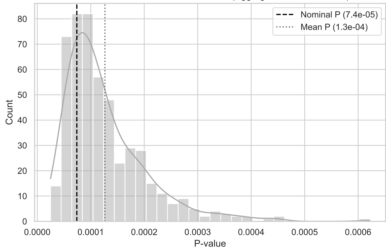
MC Distribution of P-values for T Area (Aggregated BottomLeft YZ)
