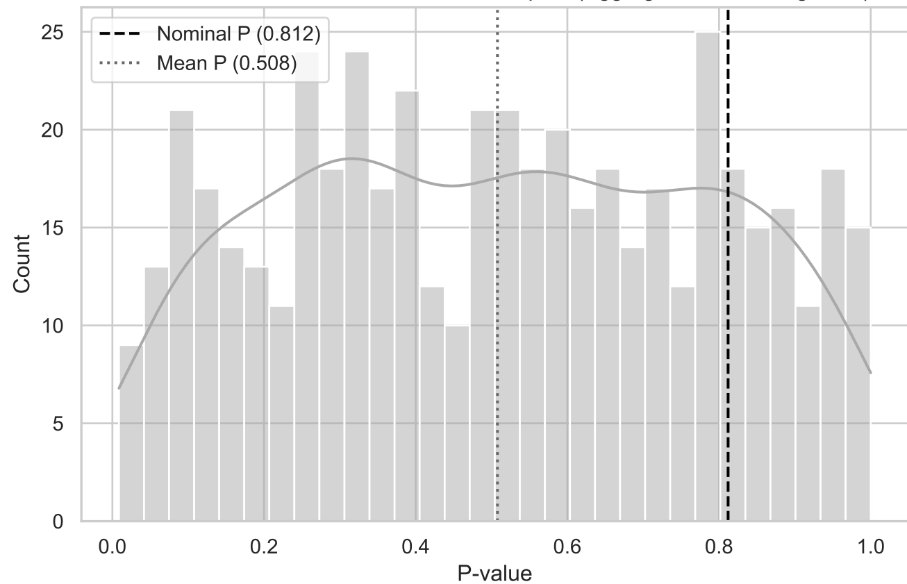
MC Distribution of P-values for QRS Compact (Aggregated BottomRight XY)
