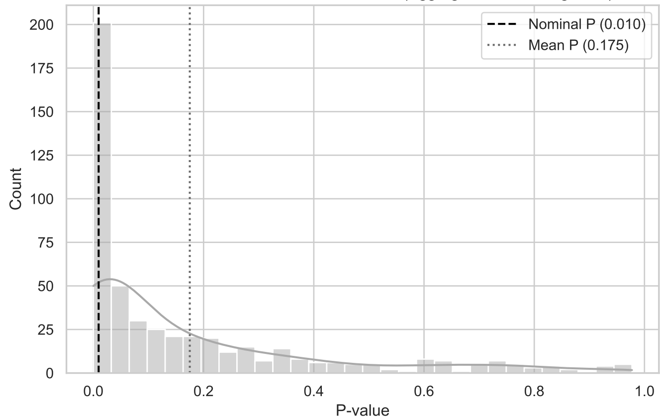
MC Distribution of P-values for ST T-Dist (Aggregated BottomRight XY)
