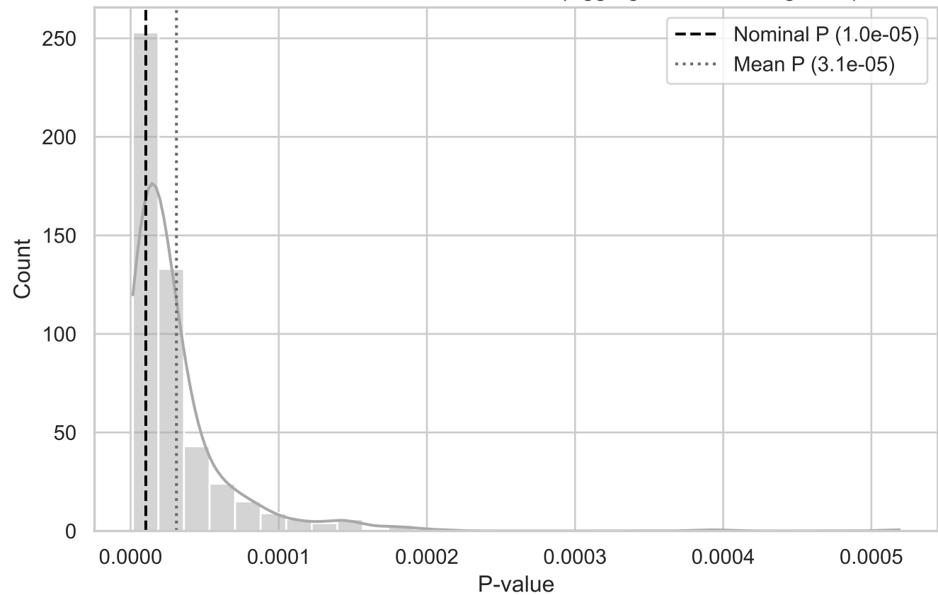
MC Distribution of P-values for T Area (Aggregated BottomRight XY)
