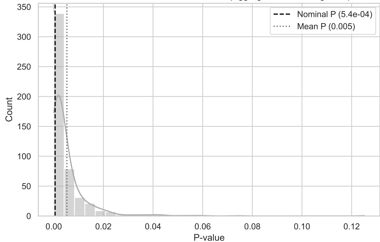
MC Distribution of P-values for T T-Dist (Aggregated BottomRight XY)
