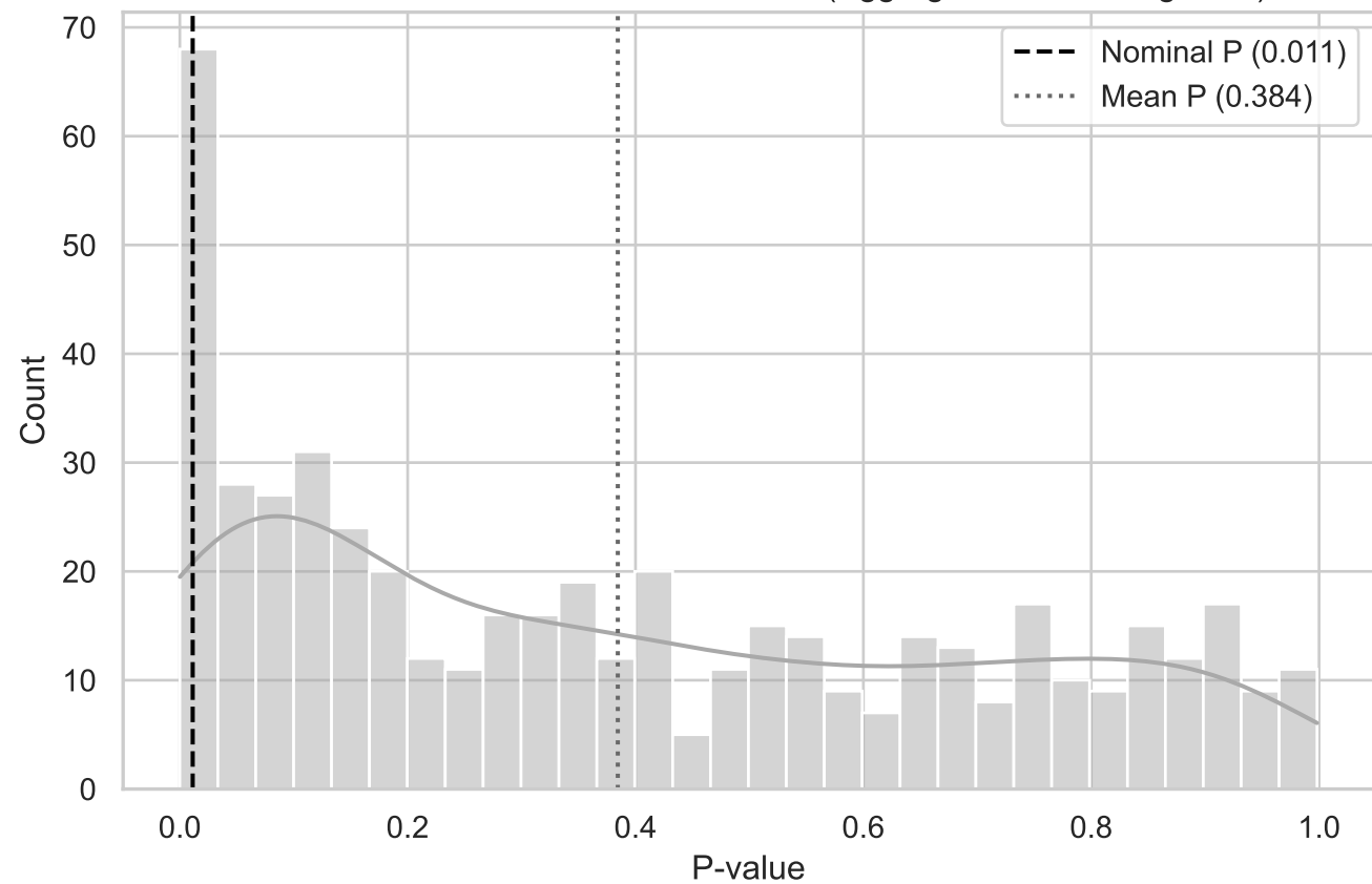
MC Distribution of P-values for ST Area (Aggregated BottomRight YZ)
