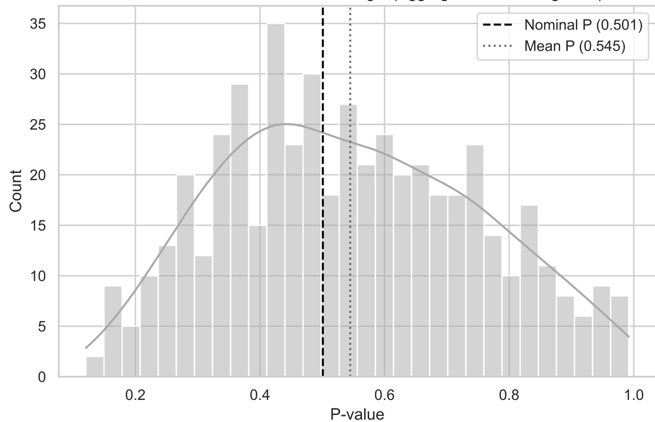
MC Distribution of P-values for T Angle (Aggregated BottomRight YZ)
