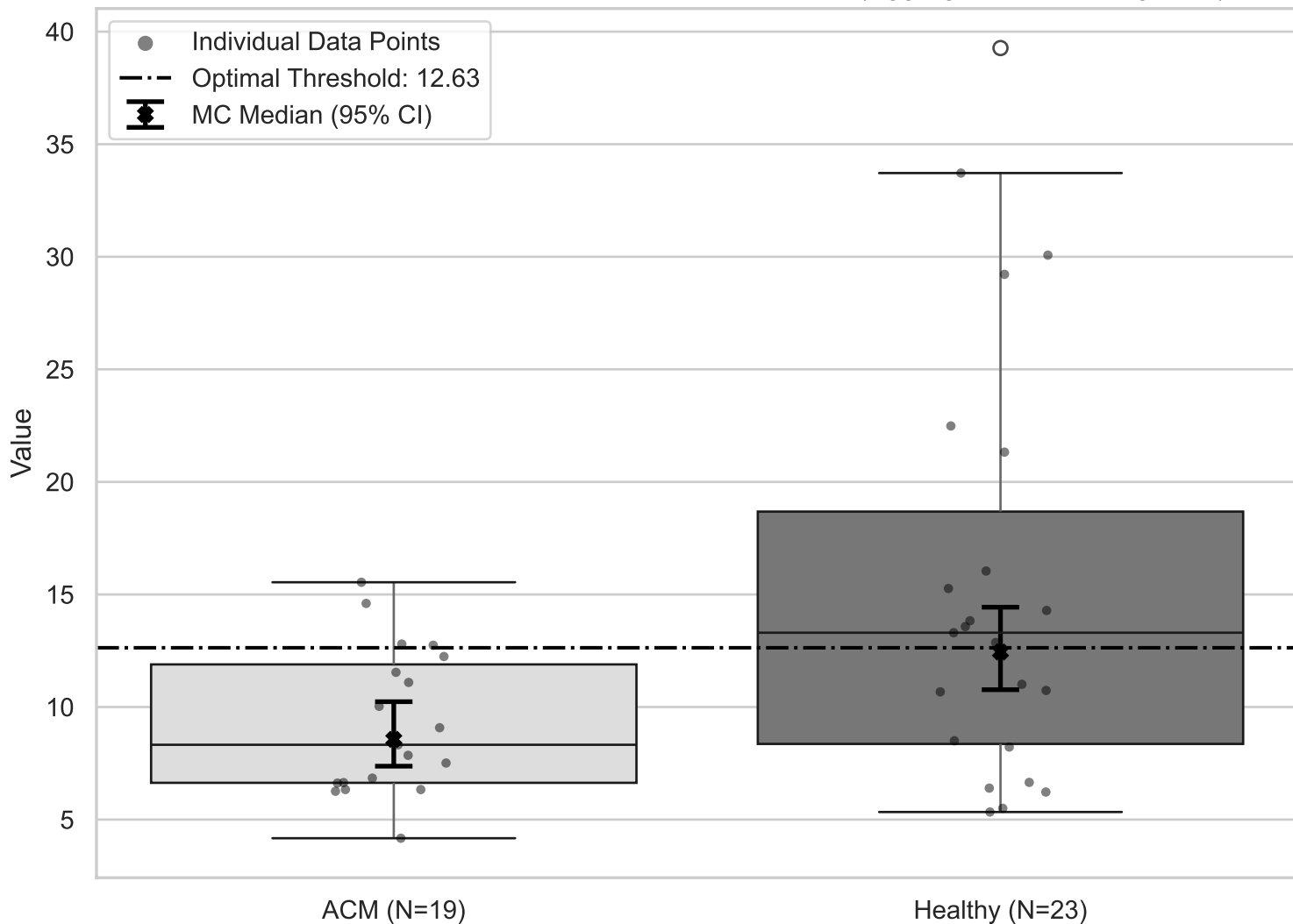
Box Plot of Nominal Data with MC Medians for T T-Dist (Aggregated BottomRight YZ)
