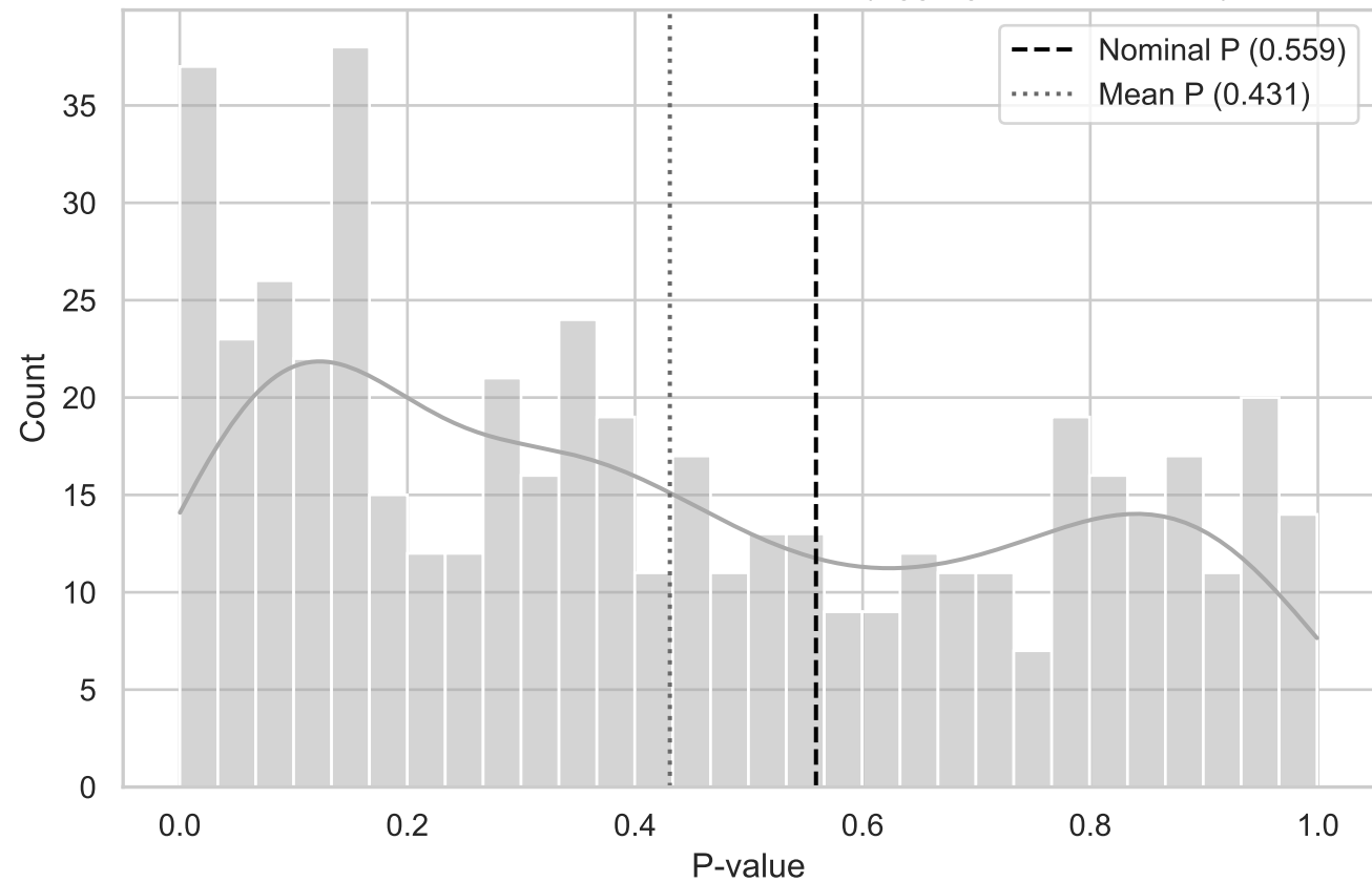
MC Distribution of P-values for ST Area (Aggregated TopLeft XY)
