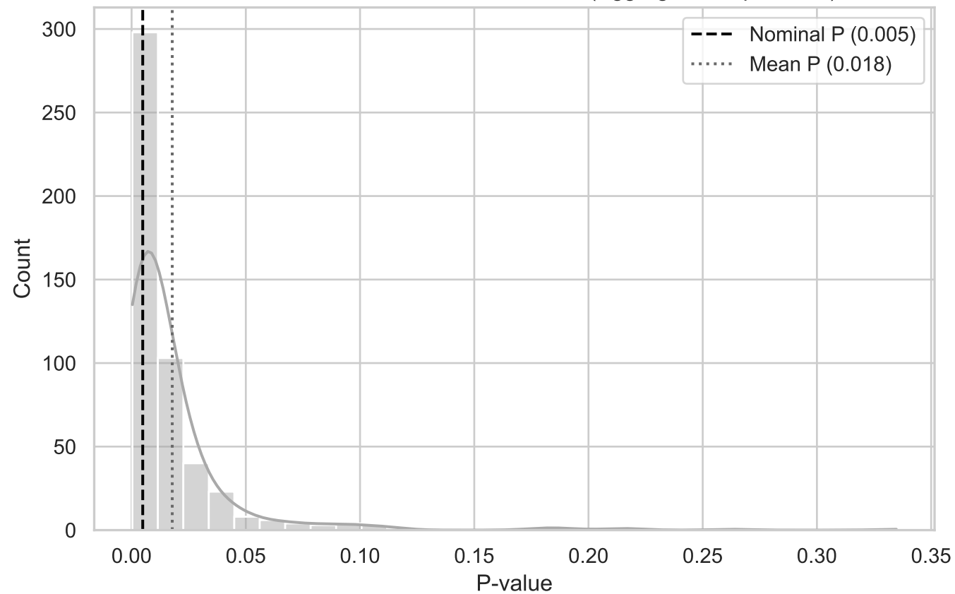
MC Distribution of P-values for T T-Dist (Aggregated TopLeft XY)
