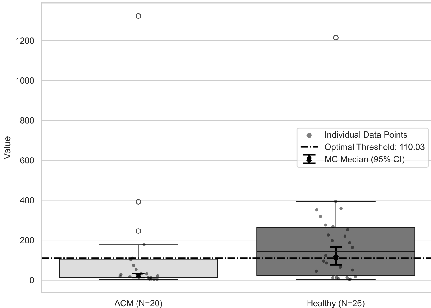
Box Plot of Nominal Data with MC Medians for QRS Area (Aggregated TopLeft YZ)
