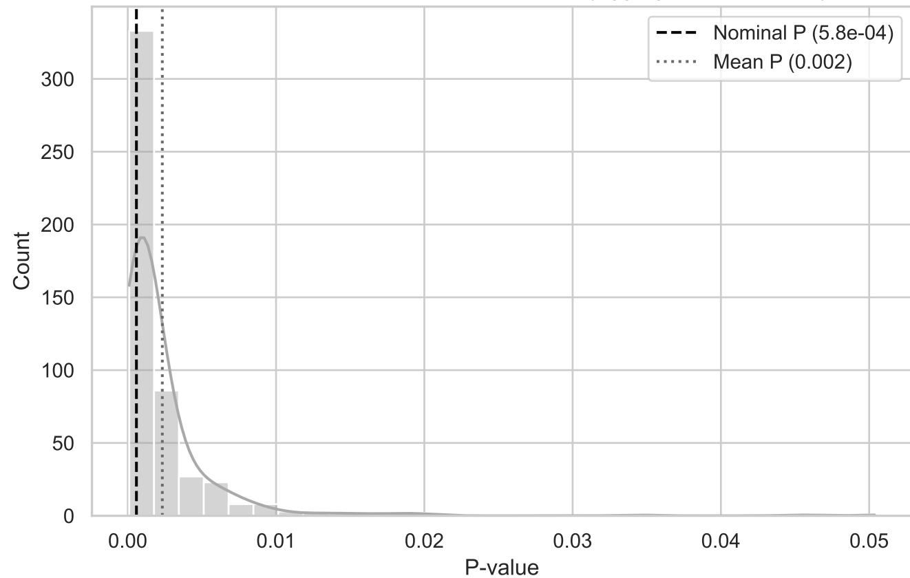
MC Distribution of P-values for QRS Area (Aggregated TopLeft YZ)
