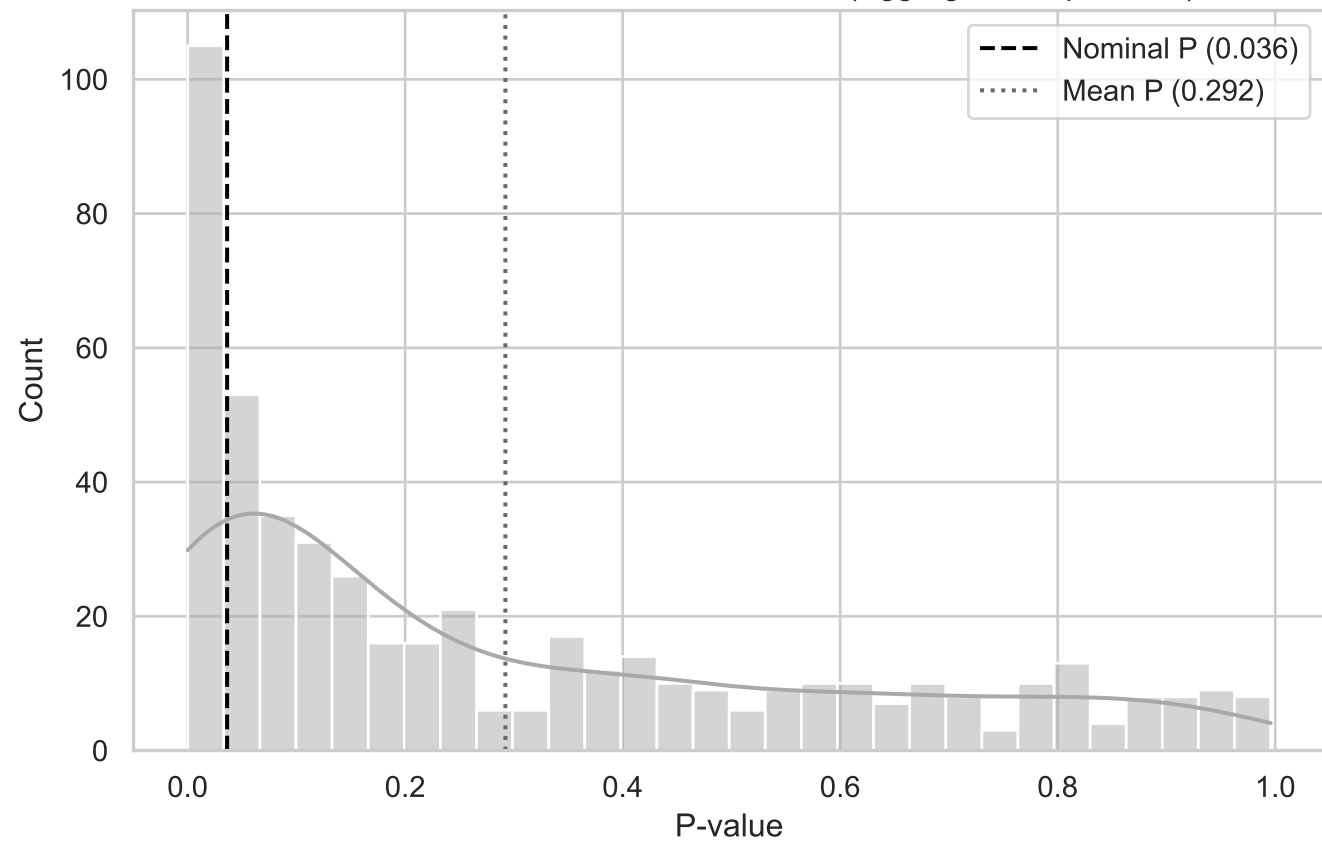
MC Distribution of P-values for ST T-Dist (Aggregated TopLeft YZ)
