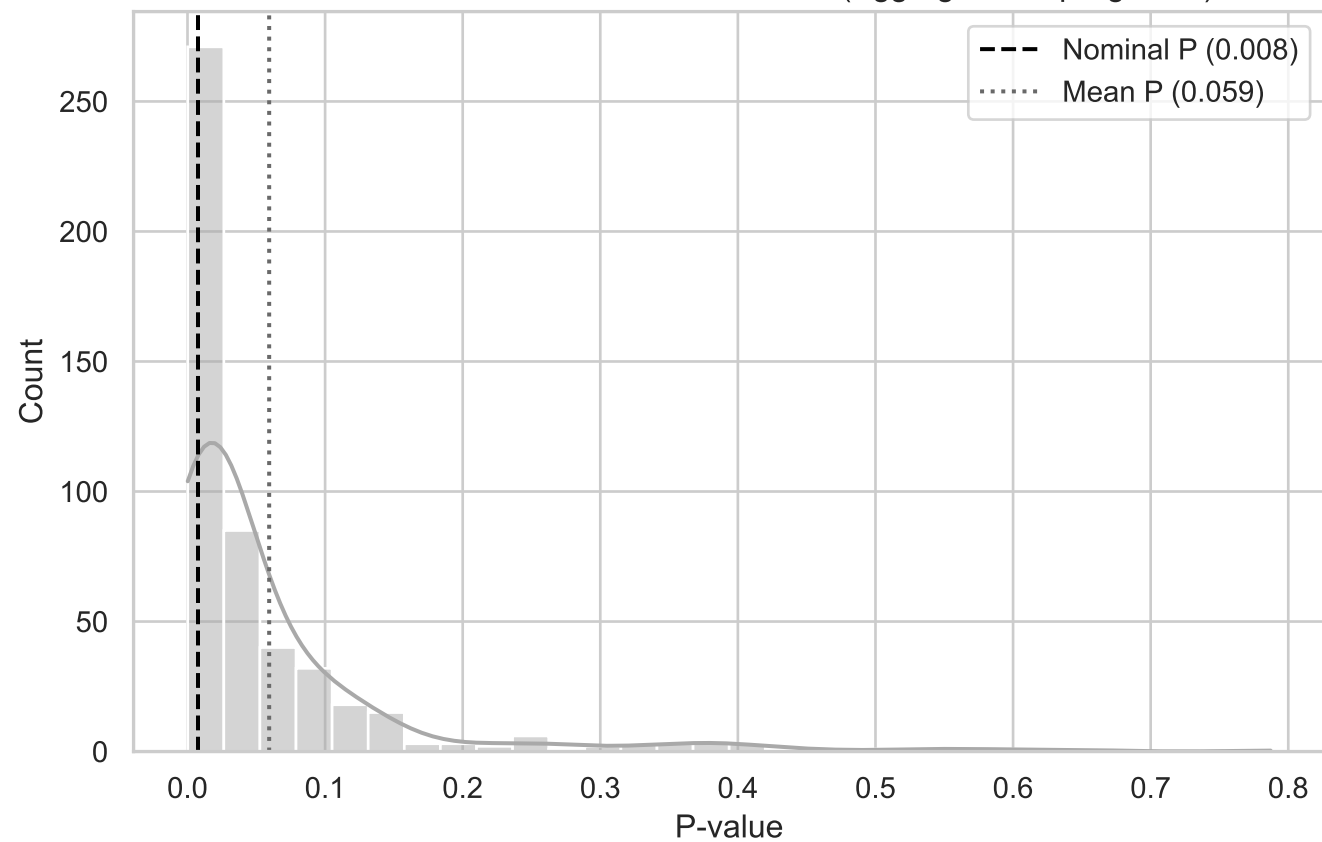
MC Distribution of P-values for QRS Area (Aggregated TopRight XY)
