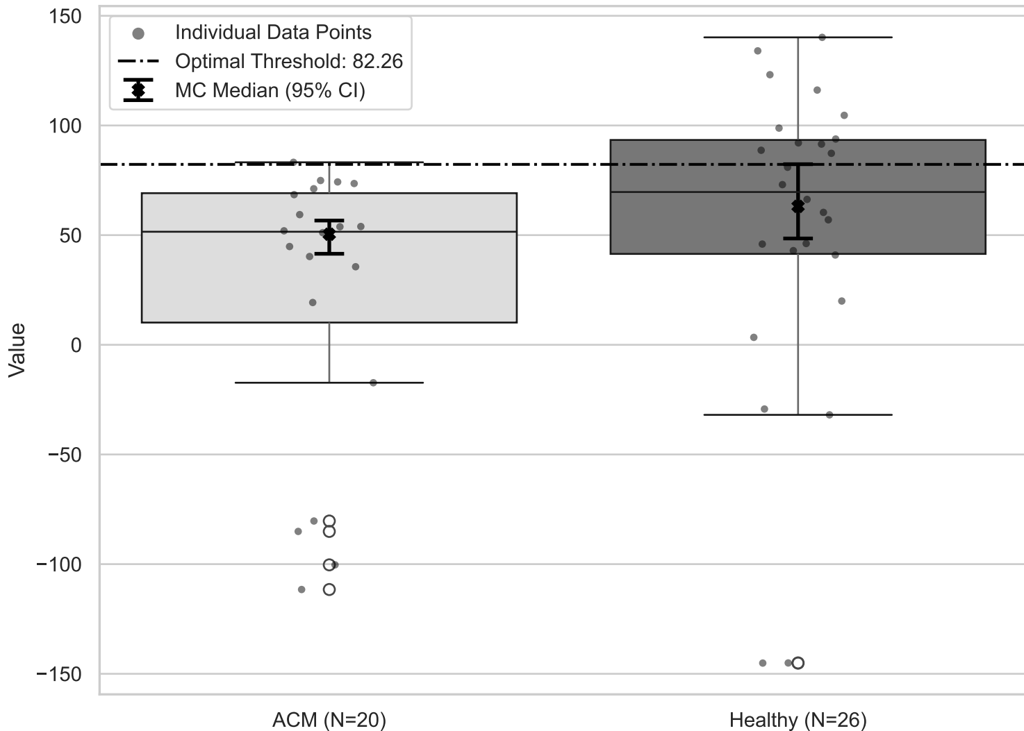
Box Plot of Nominal Data with MC Medians for ST Angle (Aggregated TopRight XY)
