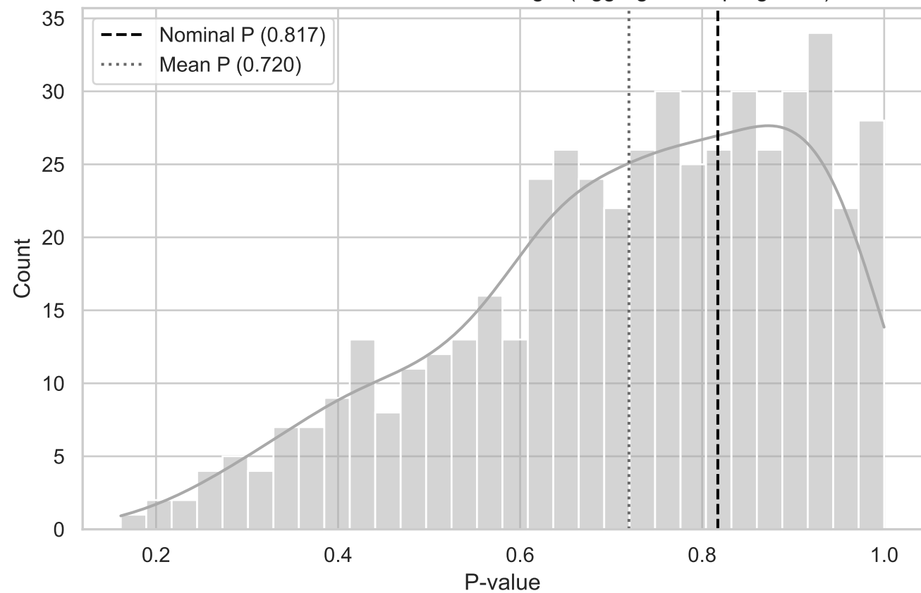
MC Distribution of P-values for T Angle (Aggregated TopRight XY)
