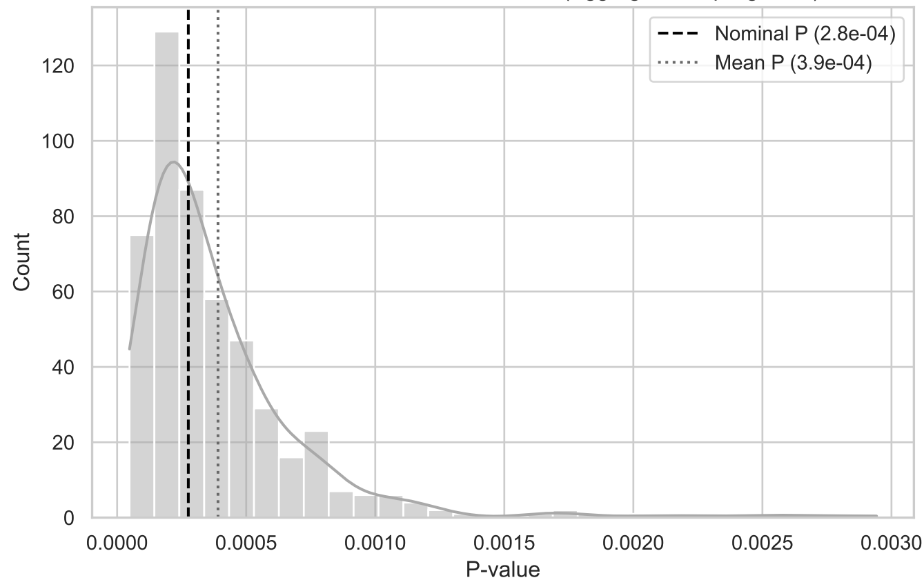
MC Distribution of P-values for T Area (Aggregated TopRight XY)
