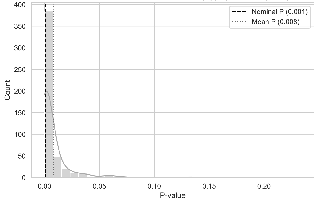
MC Distribution of P-values for QRS T-Dist (Aggregated TopRight YZ)
