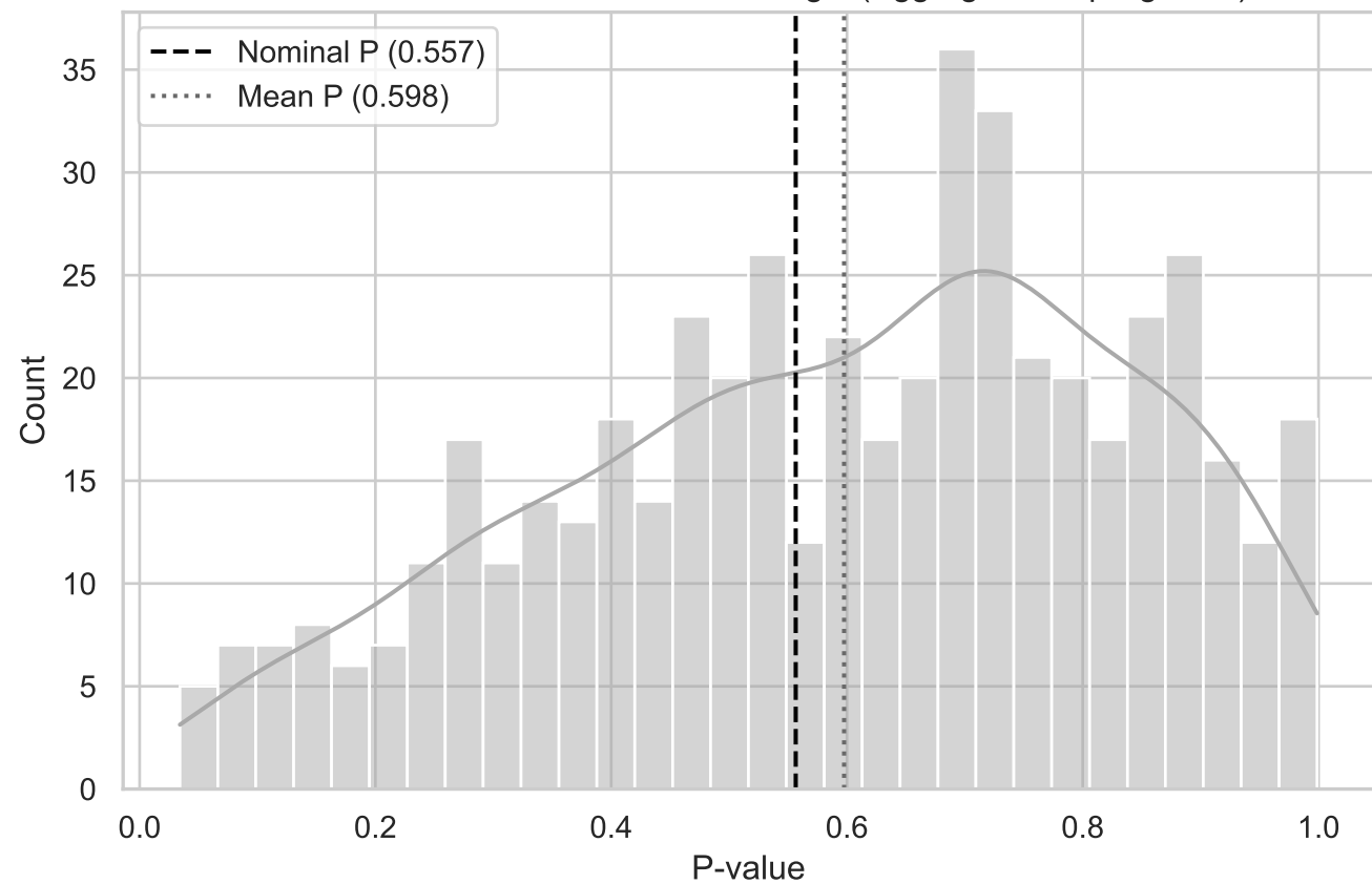
MC Distribution of P-values for ST Angle (Aggregated TopRight YZ)
