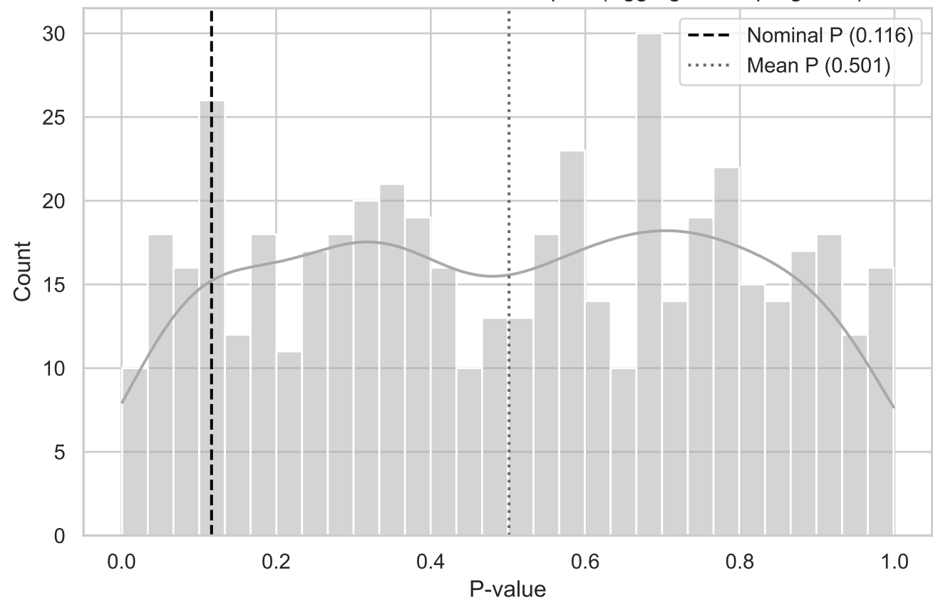
MC Distribution of P-values for ST Compact (Aggregated TopRight YZ)
