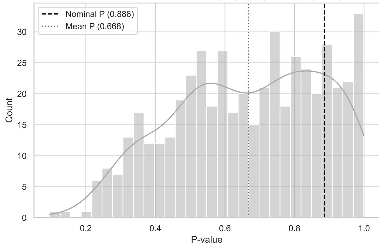
MC Distribution of P-values for T Angle (Aggregated TopRight YZ)
