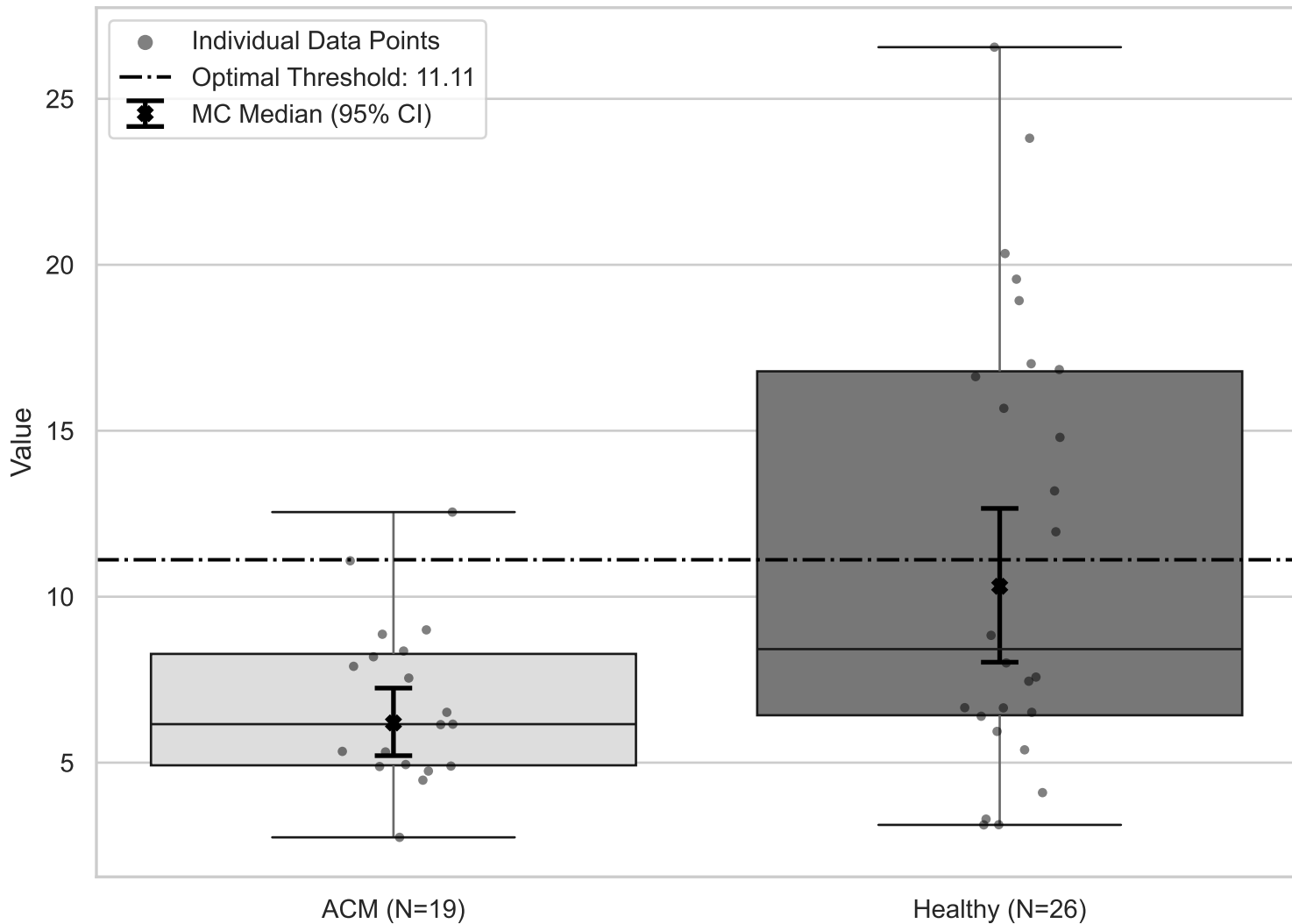
Box Plot of Nominal Data with MC Medians for T T-Dist (Aggregated TopRight YZ)
