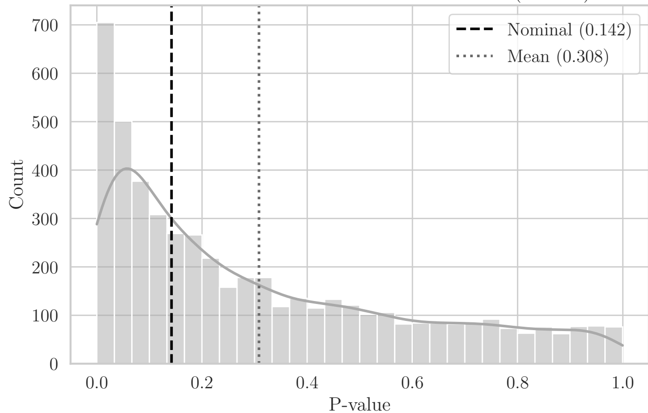
MC Distribution of P-values for ST T-Dist (C1 XY)
