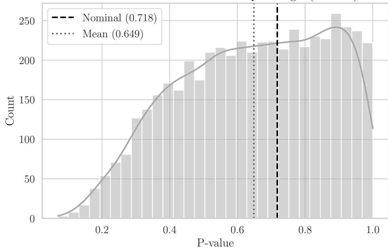
MC Distribution of P-values for QRS Angle (EY XY)
