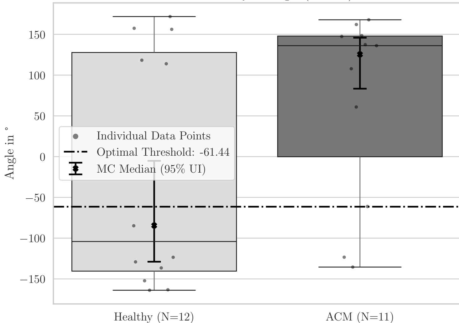
Box Plot for QRS Angle (EZ YZ)
