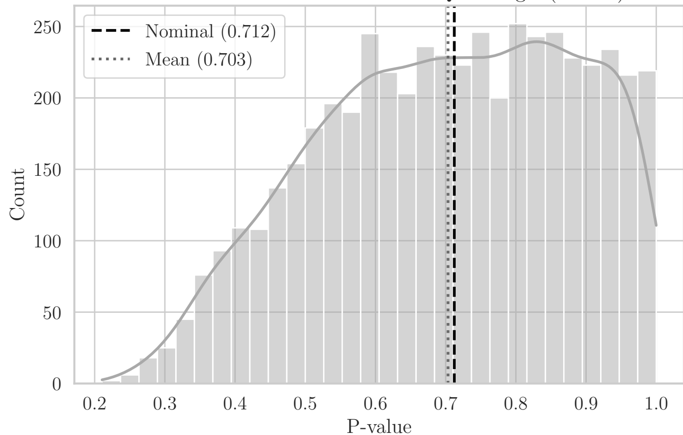
MC Distribution of P-values for QRS Angle (F0 YZ)
