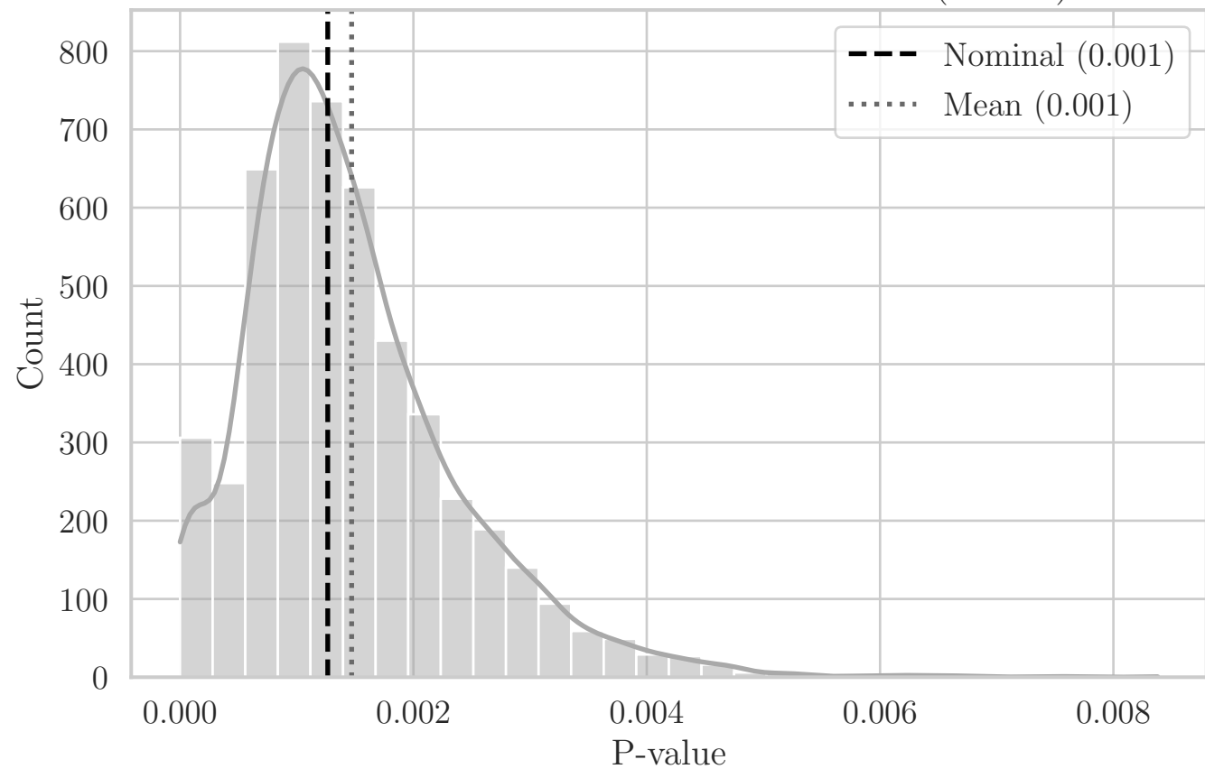
MC Distribution of P-values for T Area (F0 YZ)
