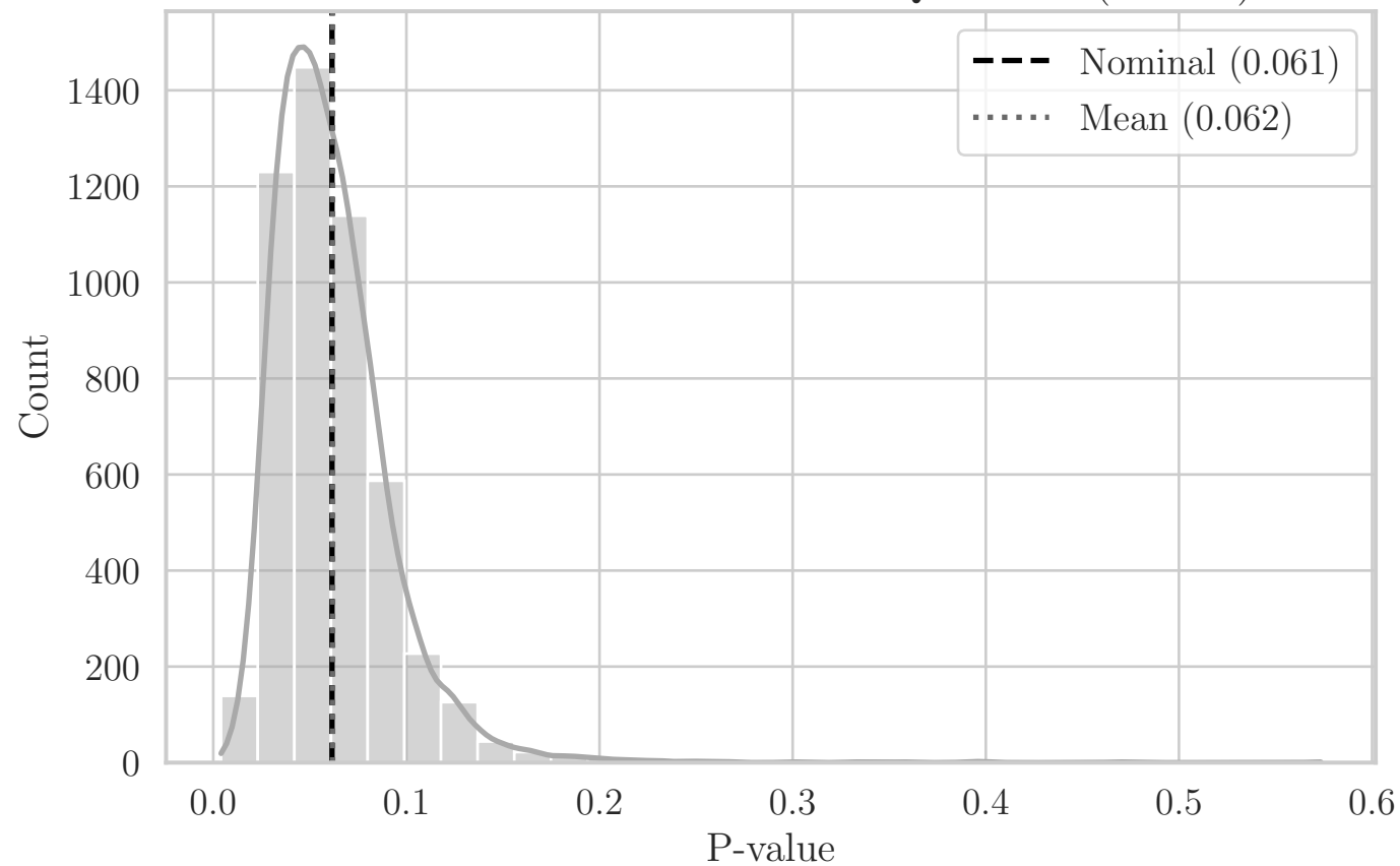
MC Distribution of P-values for QRS Area (F2 XY)
