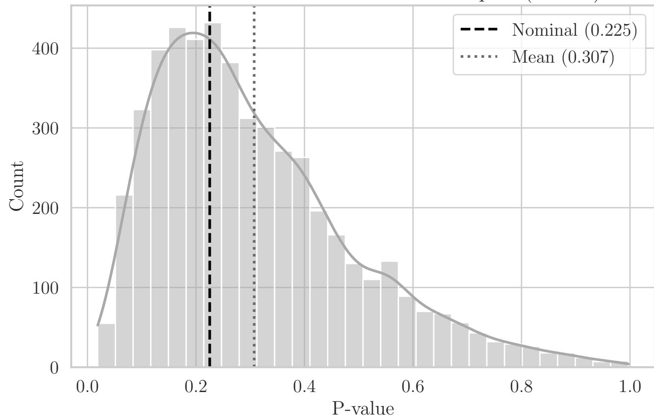
MC Distribution of P-values for T Compact (F2 XY)
